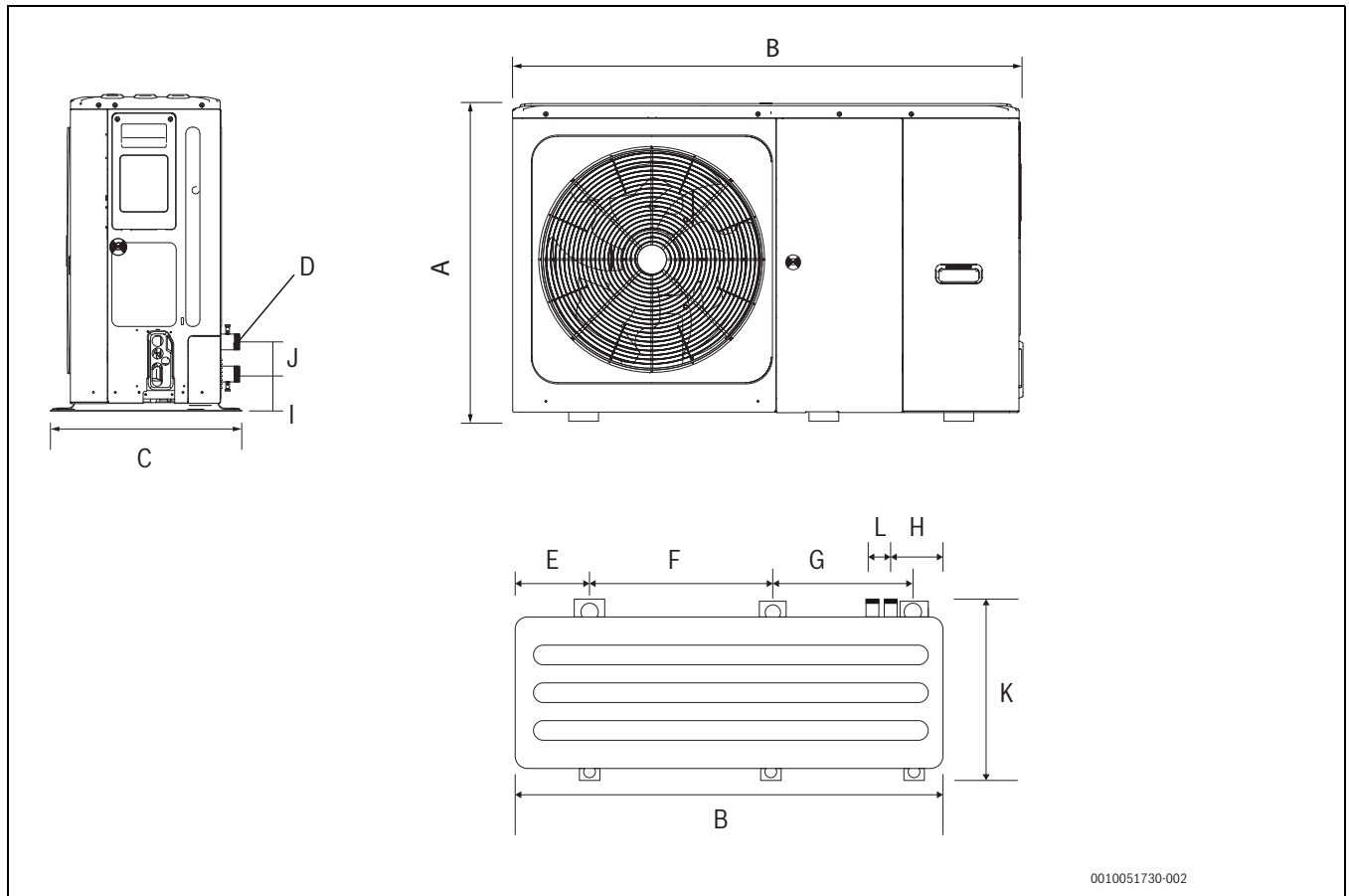
Fig. 33 Modelli da CS2000AWF 8 R-S a CS2000AWF 16 R-S/CS2000AWF 16 R-T
