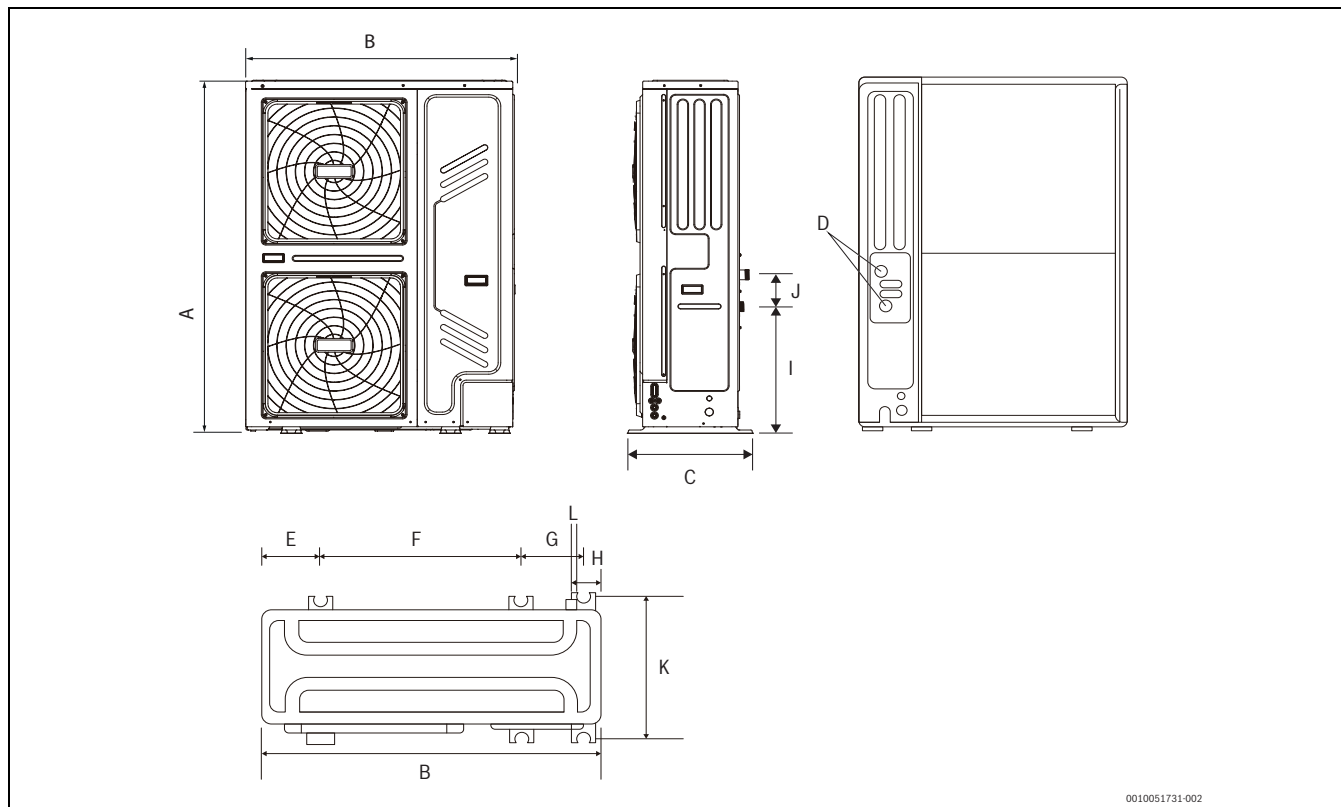
Fig. 34 Modelli da CS2000AWF 18 R-T a CS2000AWF 30 R-T
