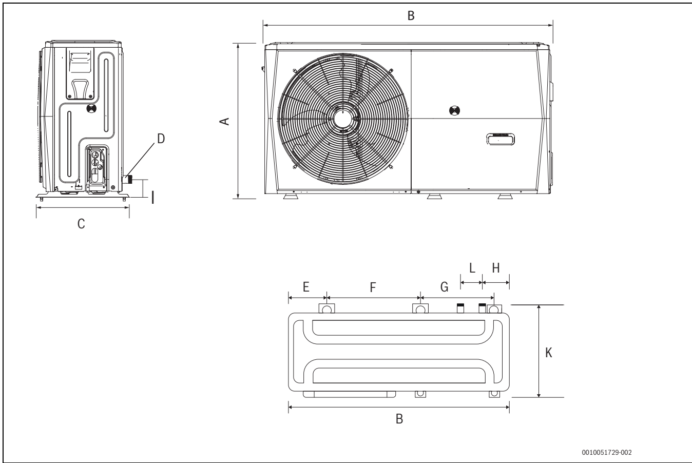
Fig. 32 Modelli da CS2000AWF 4 R-S a CS2000AWF 6 R-S
